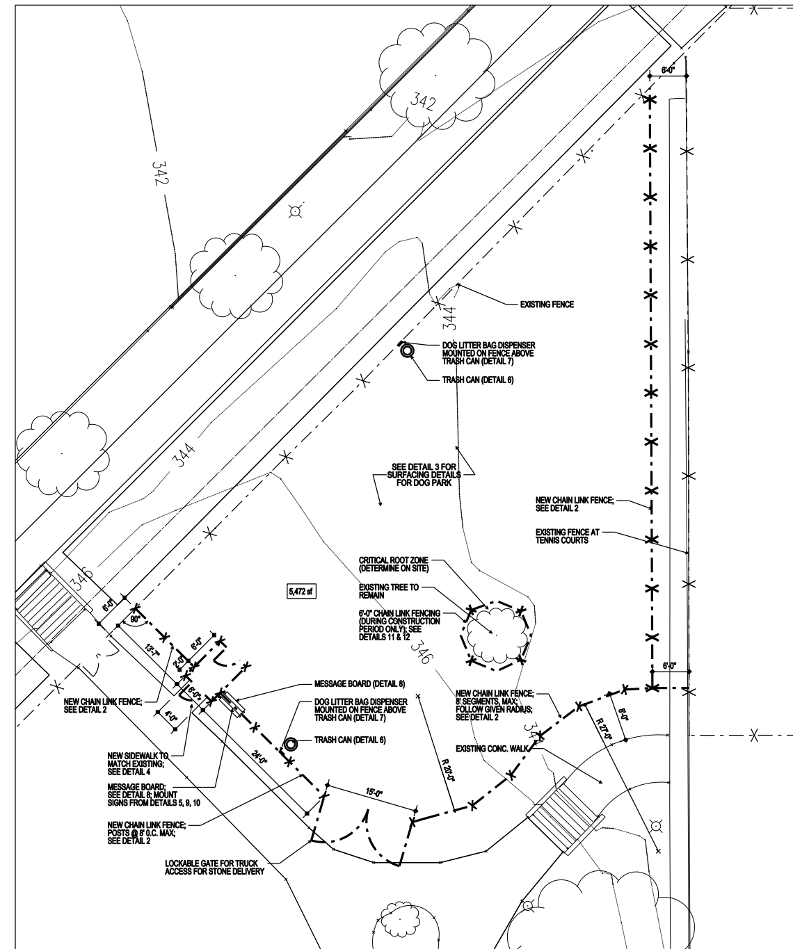
1 SITE PLAN DOG PARK SCALE: 1/8" = 1'-0"
