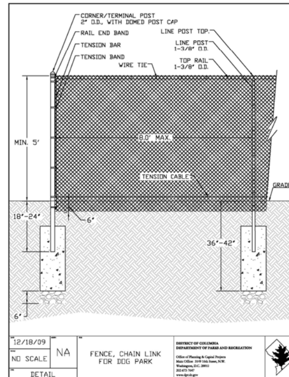
2 CHAIN LINK FENCE DETAIL SCALE: NA
