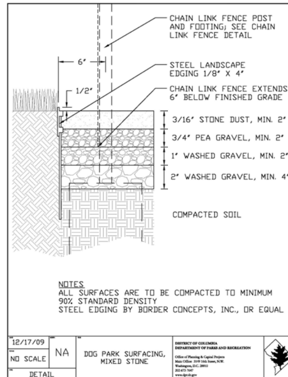
3 SURFACE DETAIL SCALE: NA
